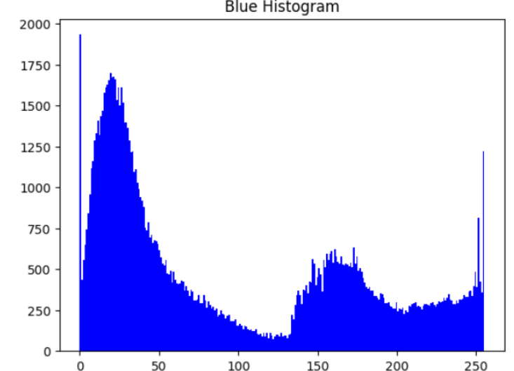
Blue Histogram
