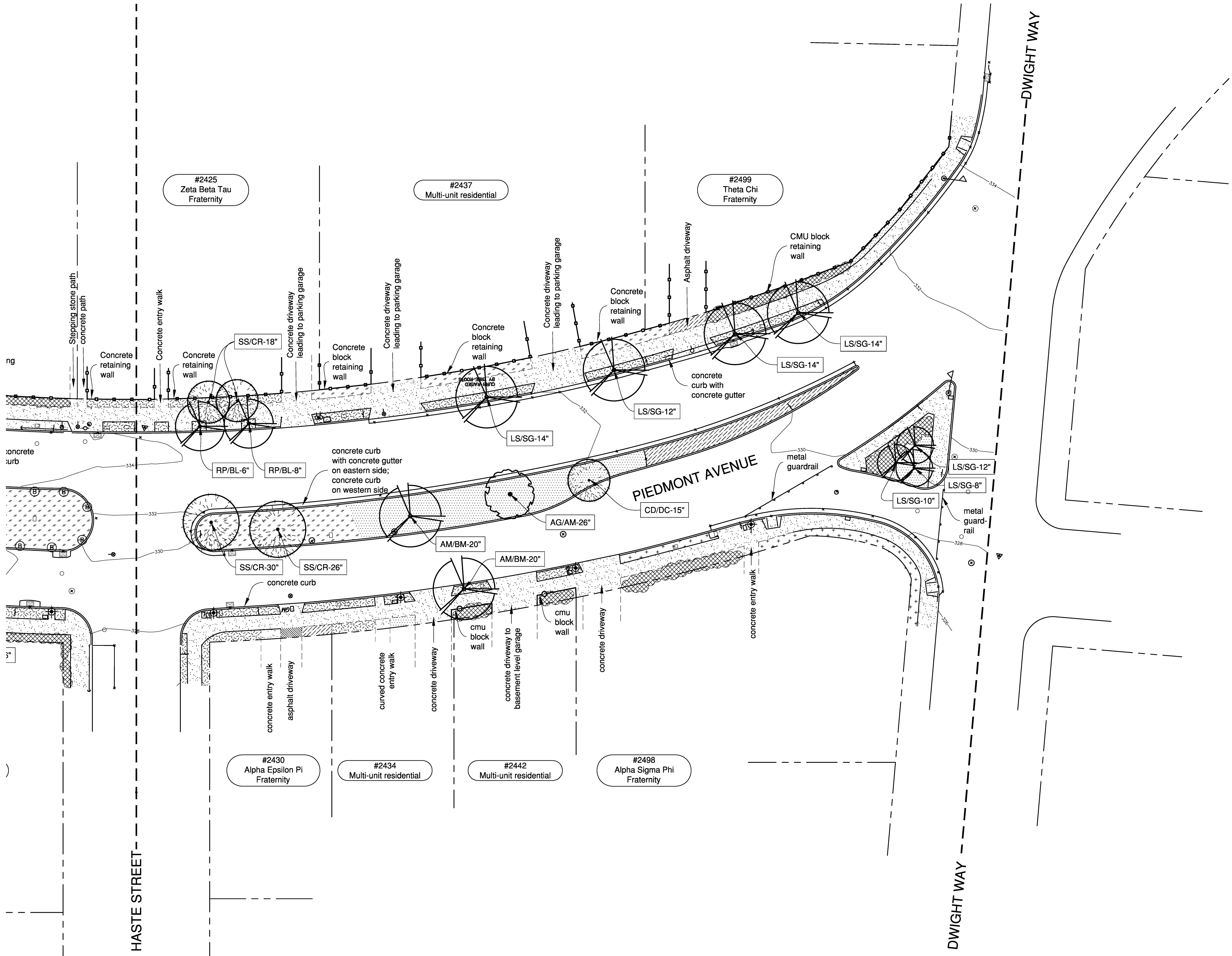
2006 Existing Conditions Plan DWIGHT WAY TO HASTE STREET
