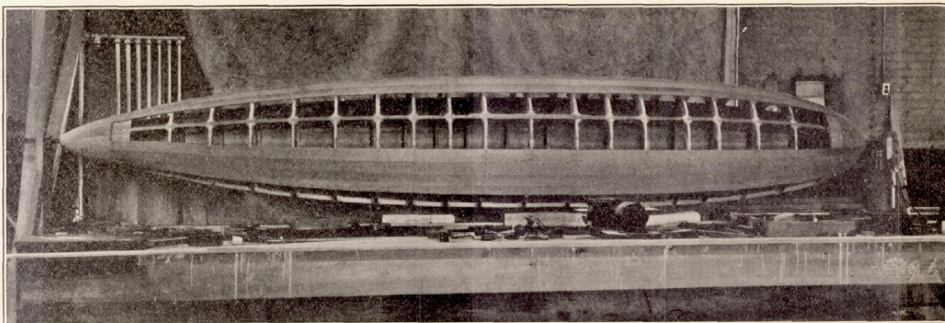
FIGURE 1.—Details of construction of the \frac{1}{40} -scale model U. S. S. Akron
