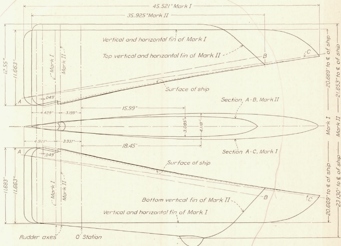
FIGURE 2.—Mark-I and Mark-II fins and control surfaces for the \frac{1}{40} -scale model U. S. S. Akron
