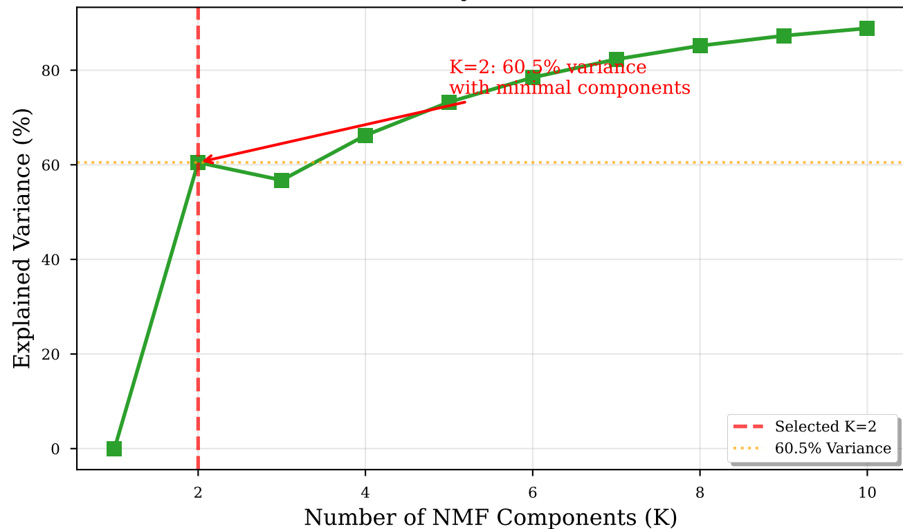
Panel B: Parsimony vs. Variance Trade-off
