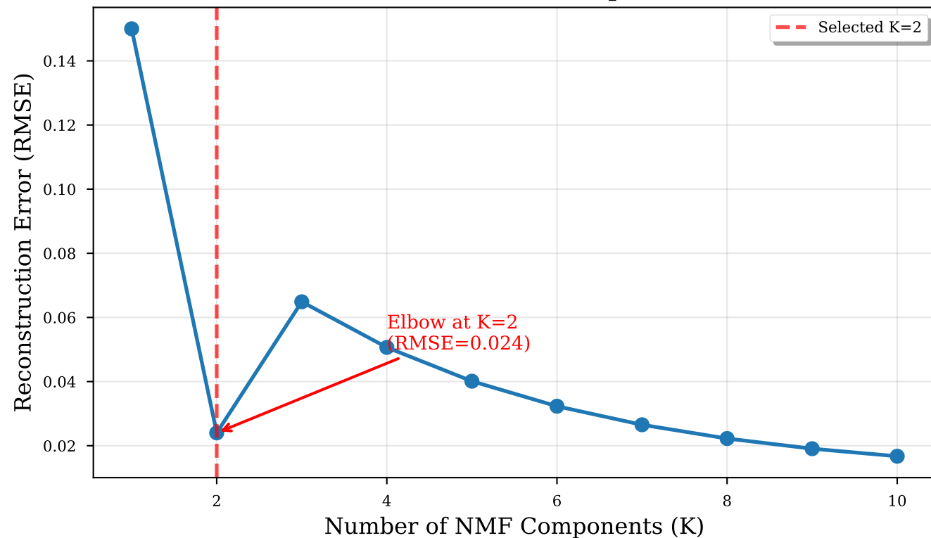
Panel A: Elbow Method for Component Selection
