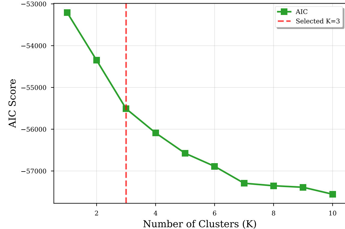
Panel B: Akaike Information Criterion
