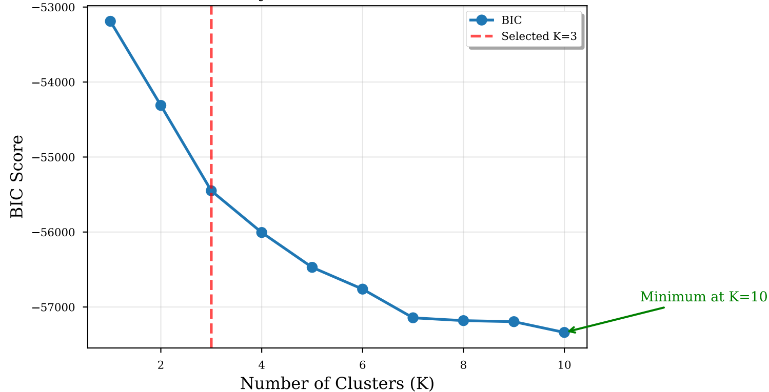
Panel A: Bayesian Information Criterion
