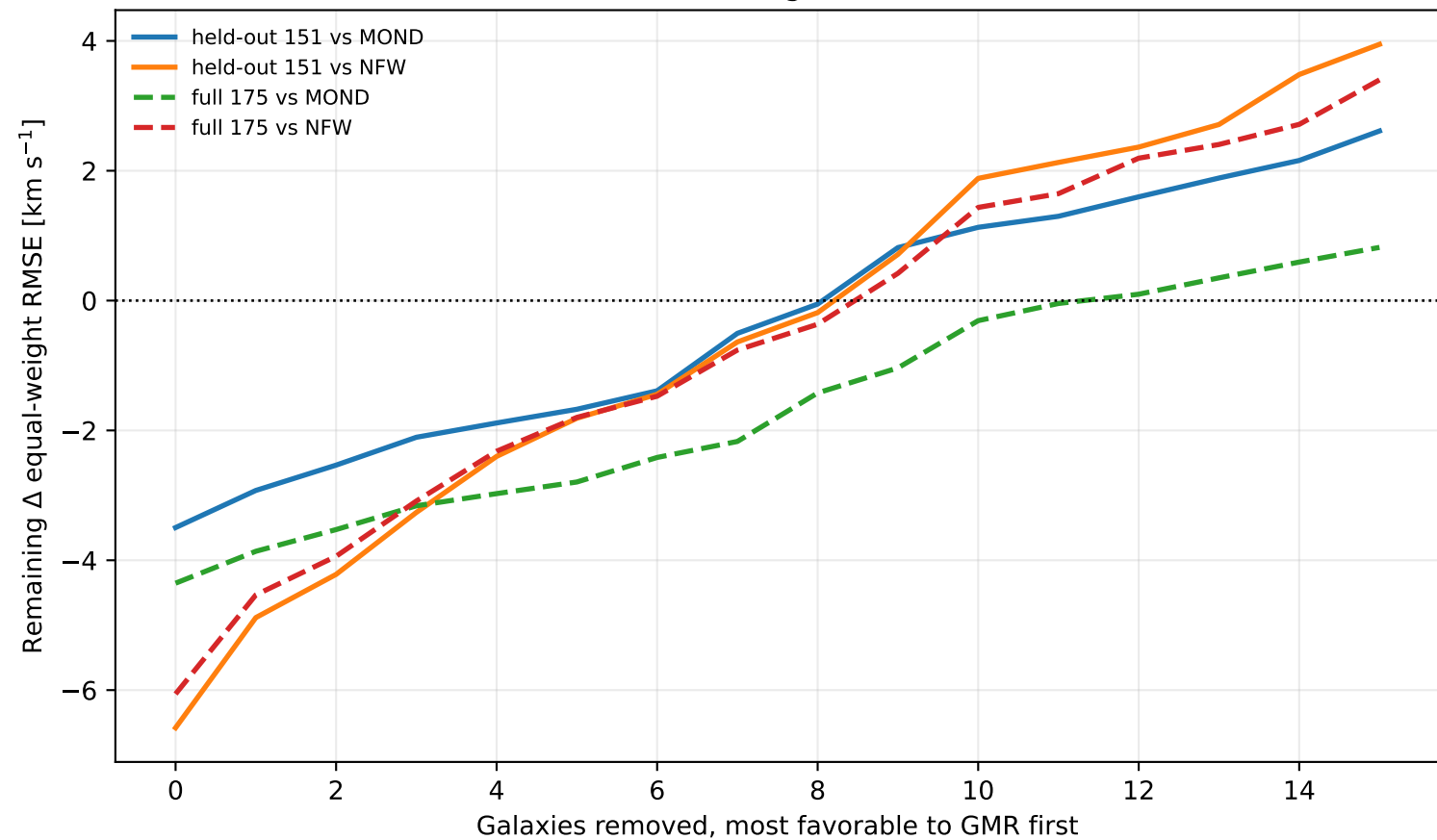
Outlier influence and sign-reversal thresholds
