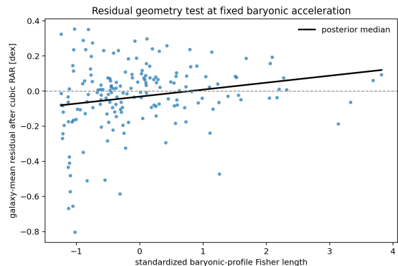
Figure 5. Galaxy-block residual-geometry test. The horizontal axis is the standardized total Fisher length of the baryonic compactness/profile vector. The vertical axis is the galaxy-mean residual after removing a cubic one-variable RAR baseline.
