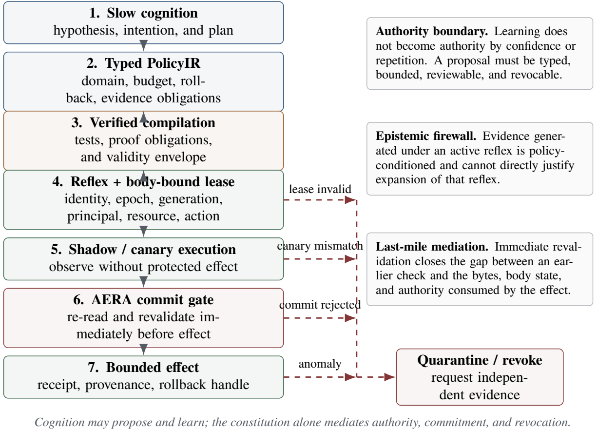
Fig. 2. Bounded cognition-to-effect pipeline. The main path converts a cognitive proposal into a typed and testable reflex. The red exception lane handles stale authority, canary mismatch, commit rejection, and post-effect anomaly without allowing evidence produced by the reflex to justify an expansion of its own authority.
