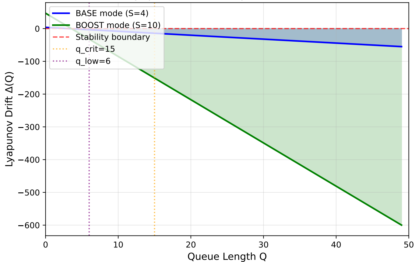
Lyapunov Drift Analysis: V(Q) = Q^2
