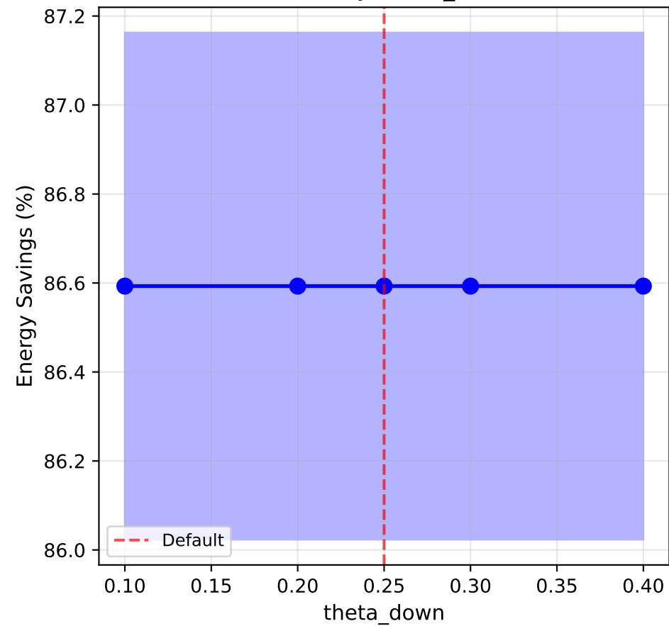
Sensitivity: theta_down
