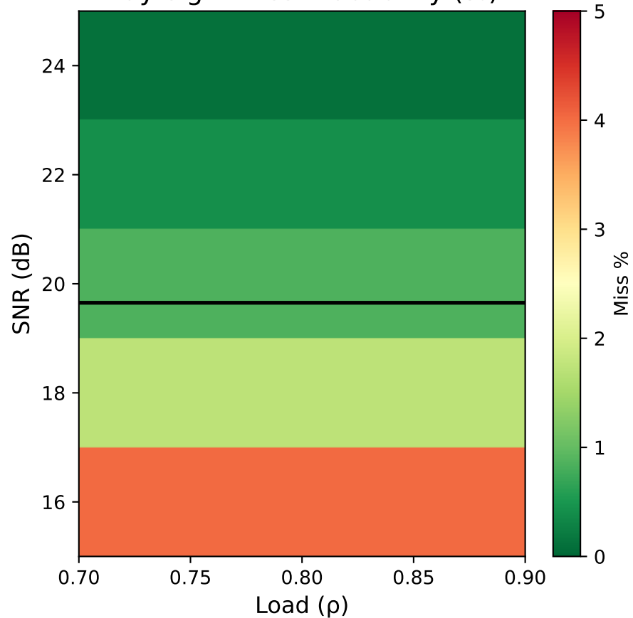
Rayleigh: Miss Probability (%)
