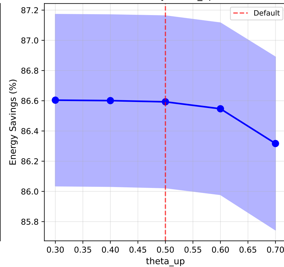
Sensitivity: theta_up
