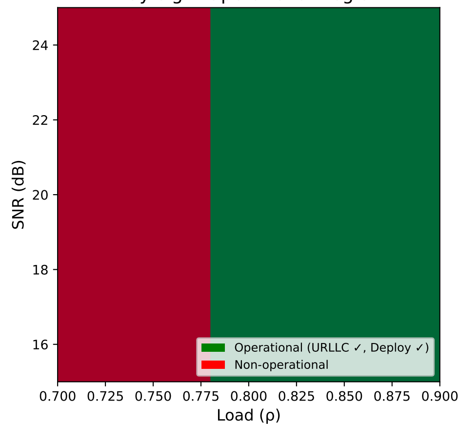
Rayleigh: Operational Region
