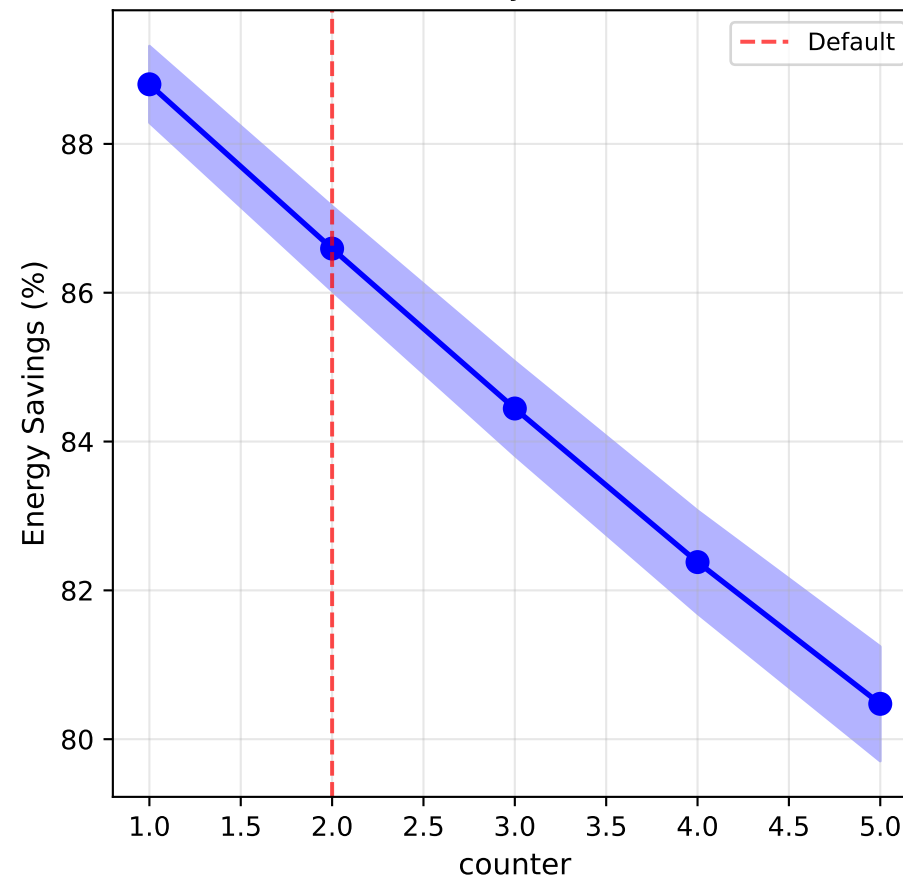
Sensitivity: counter
