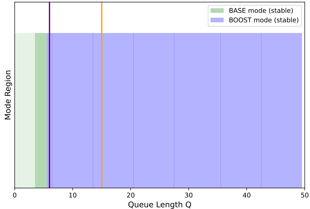
SENTRY-Lite-2 Mode Selection Regions
