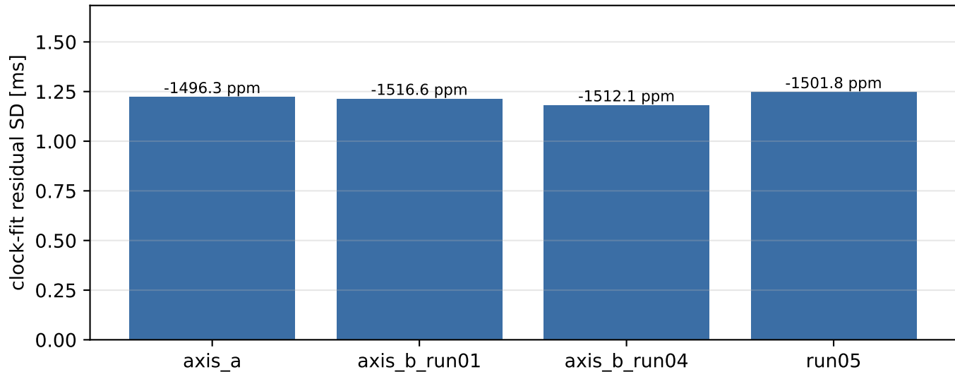
Camera ↔ motor alignment, fitted to serial motor events only (114 events per out-of-plane run)
