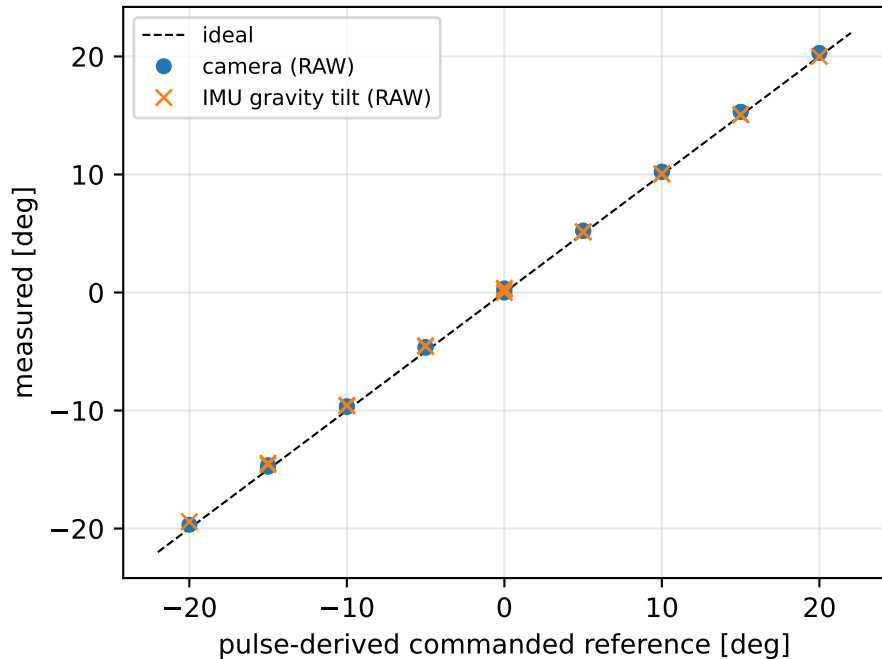
Board Y: measured vs commanded reference
