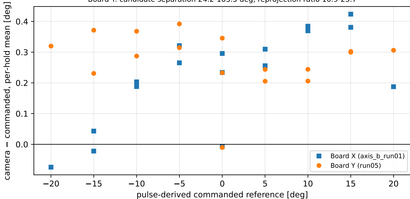
Per-hold RAW camera error, both out-of-plane axes Board Y: candidate separation 24.2-103.5 deg, reprojection ratio 10.9-23.7
