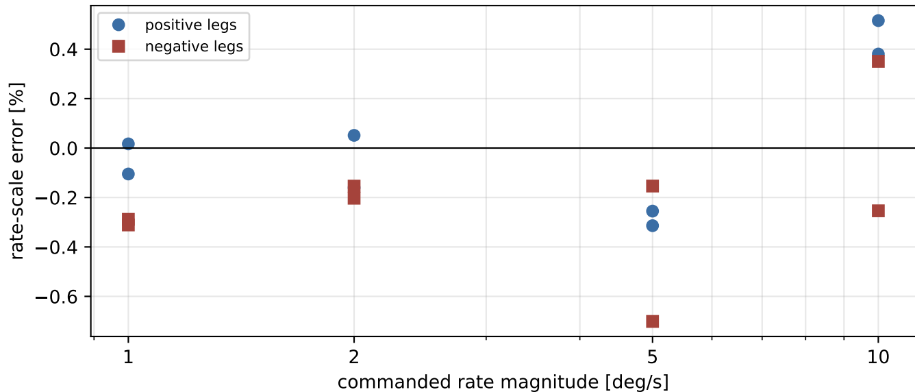
Board Y rate scale: camera displacement per leg / commanded rate (NOT an instantaneous rate RMSE)
