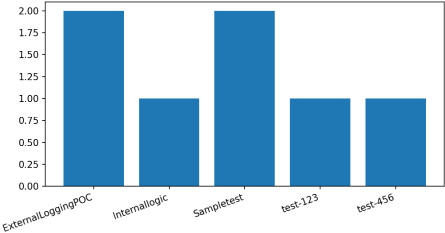
iFlow-wise Issues
