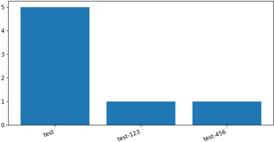
Package-wise Issues
