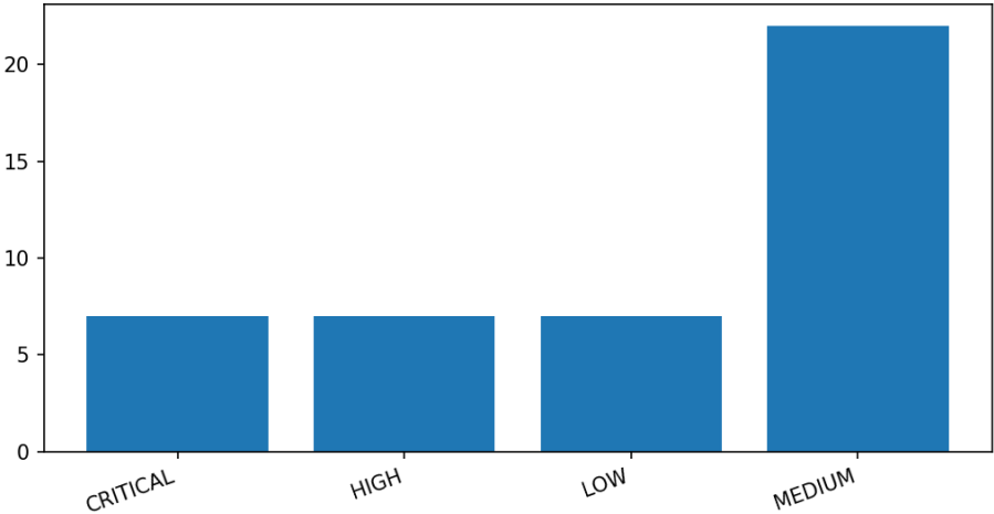
Severity Summary
