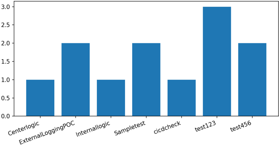
iFlow-wise Issues
