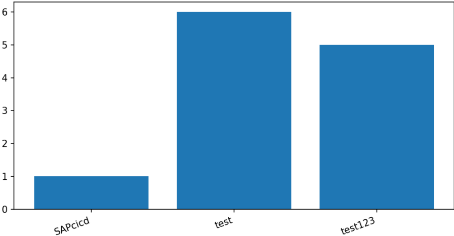
Package-wise Issues
