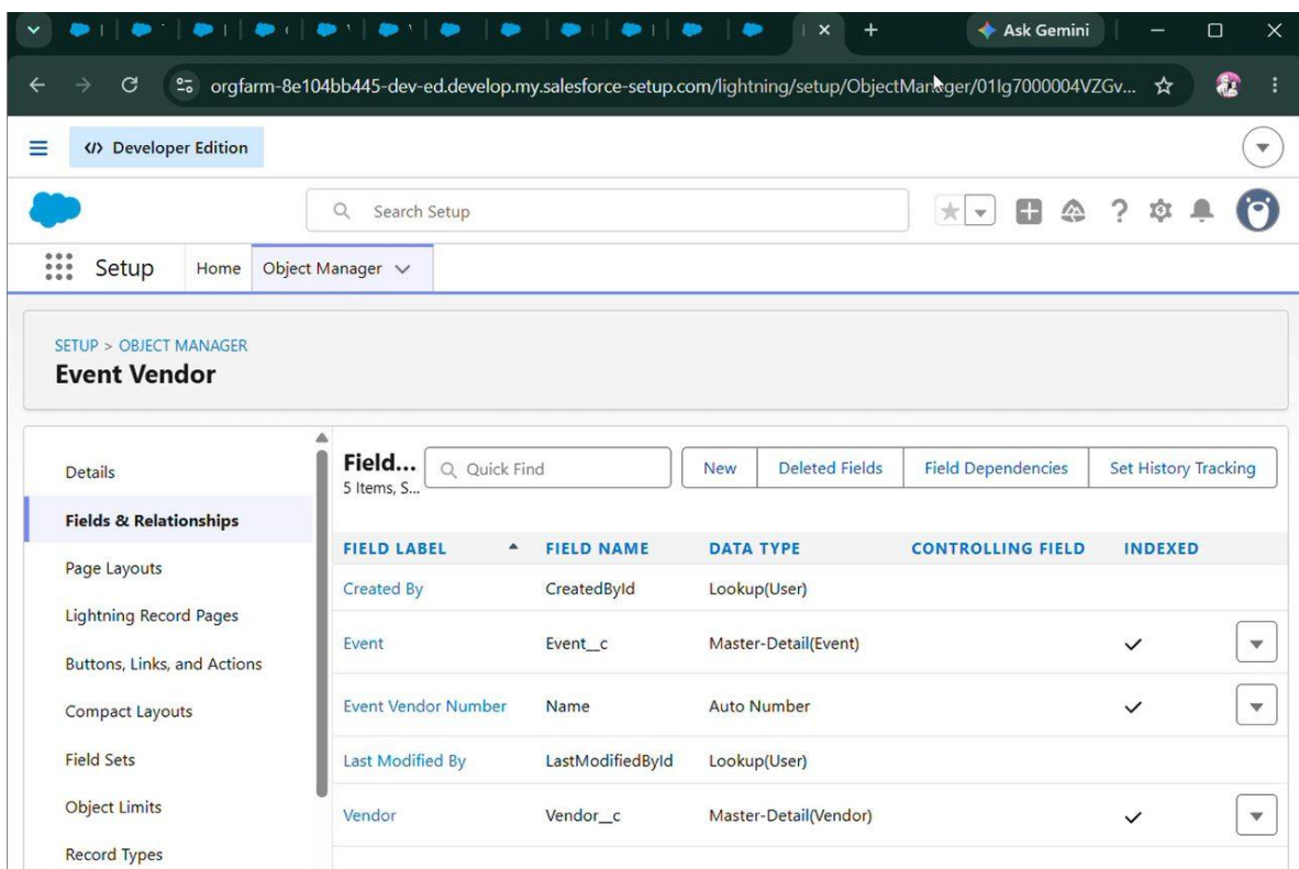
Figure 4: Event Vendor object fields and master-detail relationships
