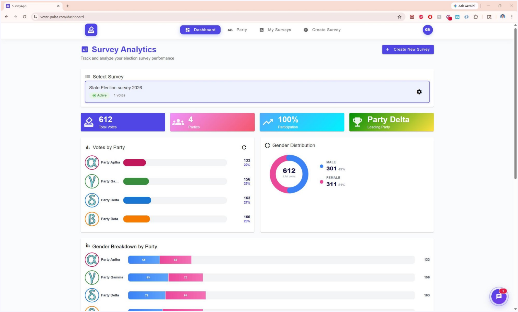
Survey Analytics Dashboard — real-time KPI cards, votes by party, gender distribution, and demographic breakdown
