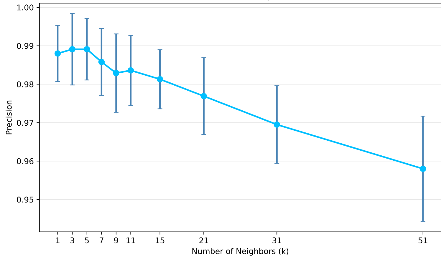
Dataset #1.1 (Hand-Written Digits): Precision vs. k
