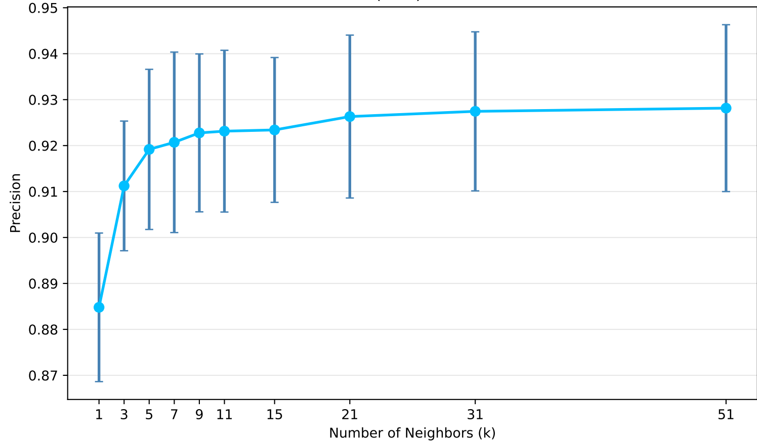
Dataset #1 (Rice): Precision vs. k
