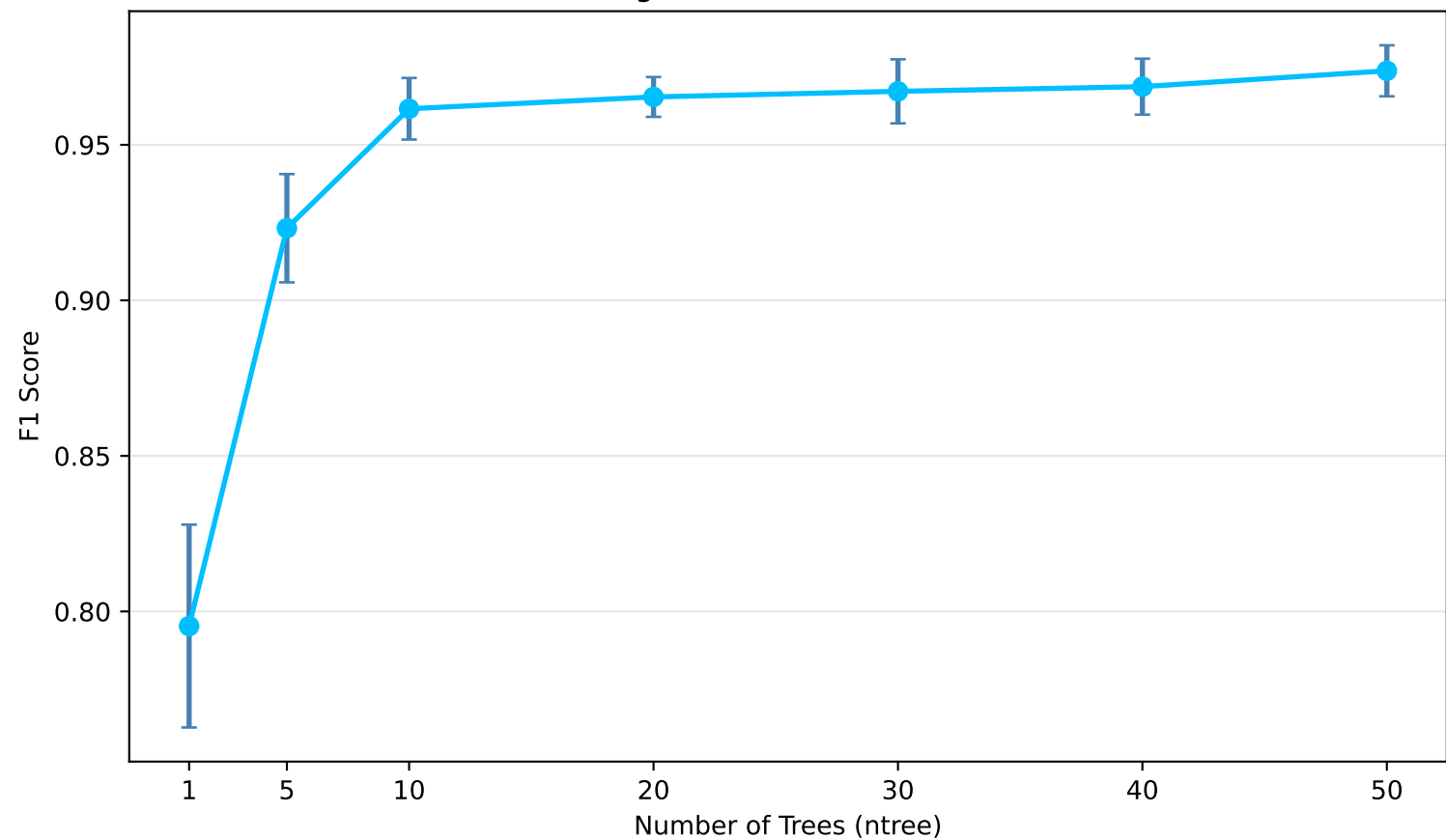
Dataset 1.1 (Digits): F1 Score vs. Number of Trees
