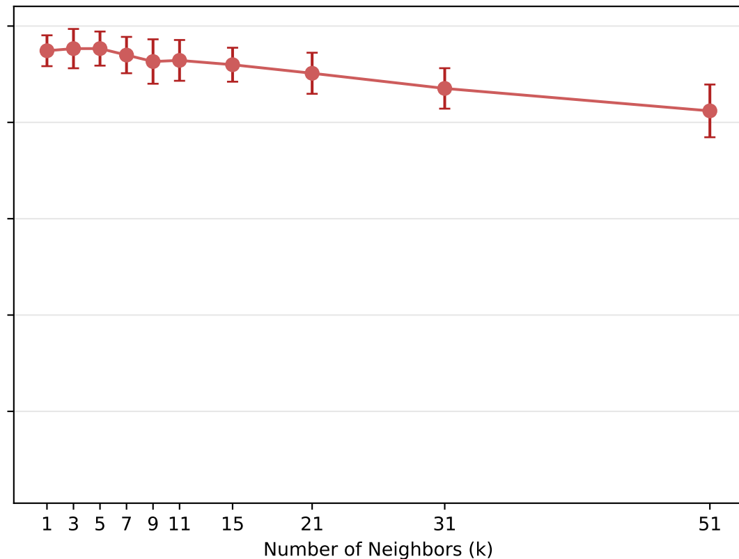
k-NN (min-max normalized)
