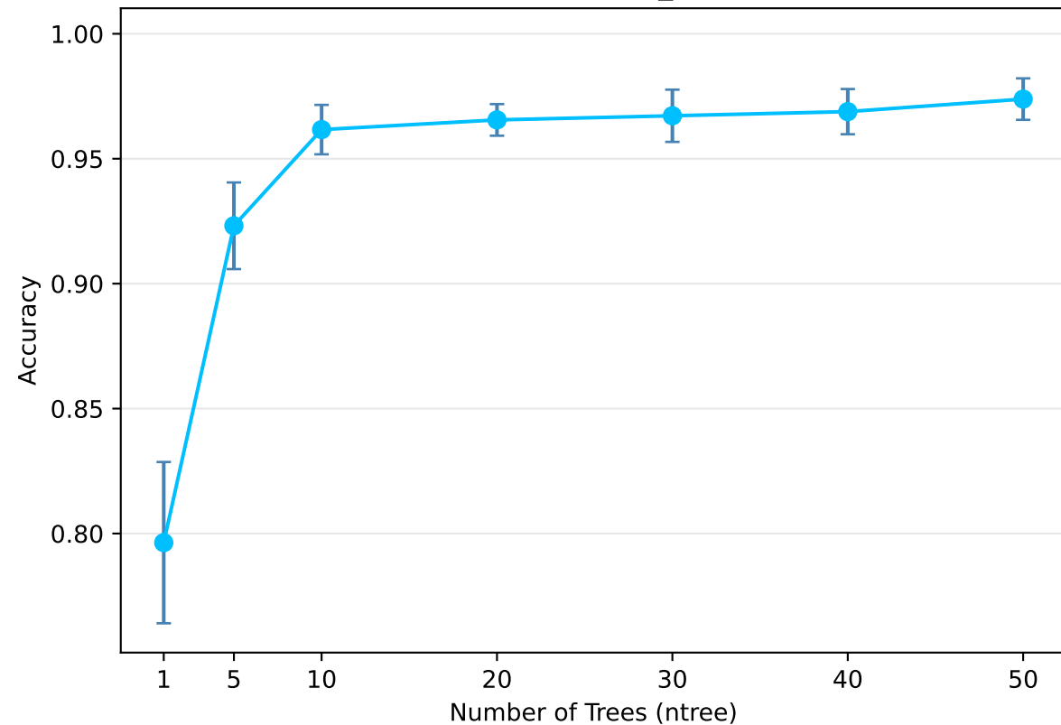
Random Forest (max_depth=10)
