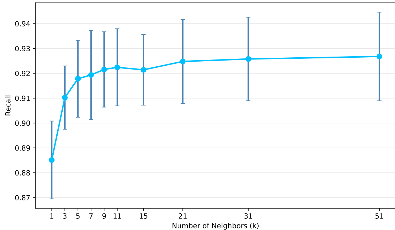
Dataset #1 (Rice): Recall vs. k
