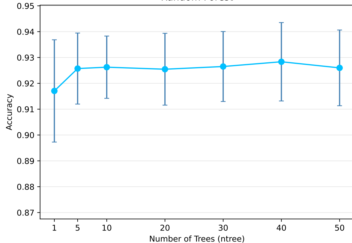
Random Forest
