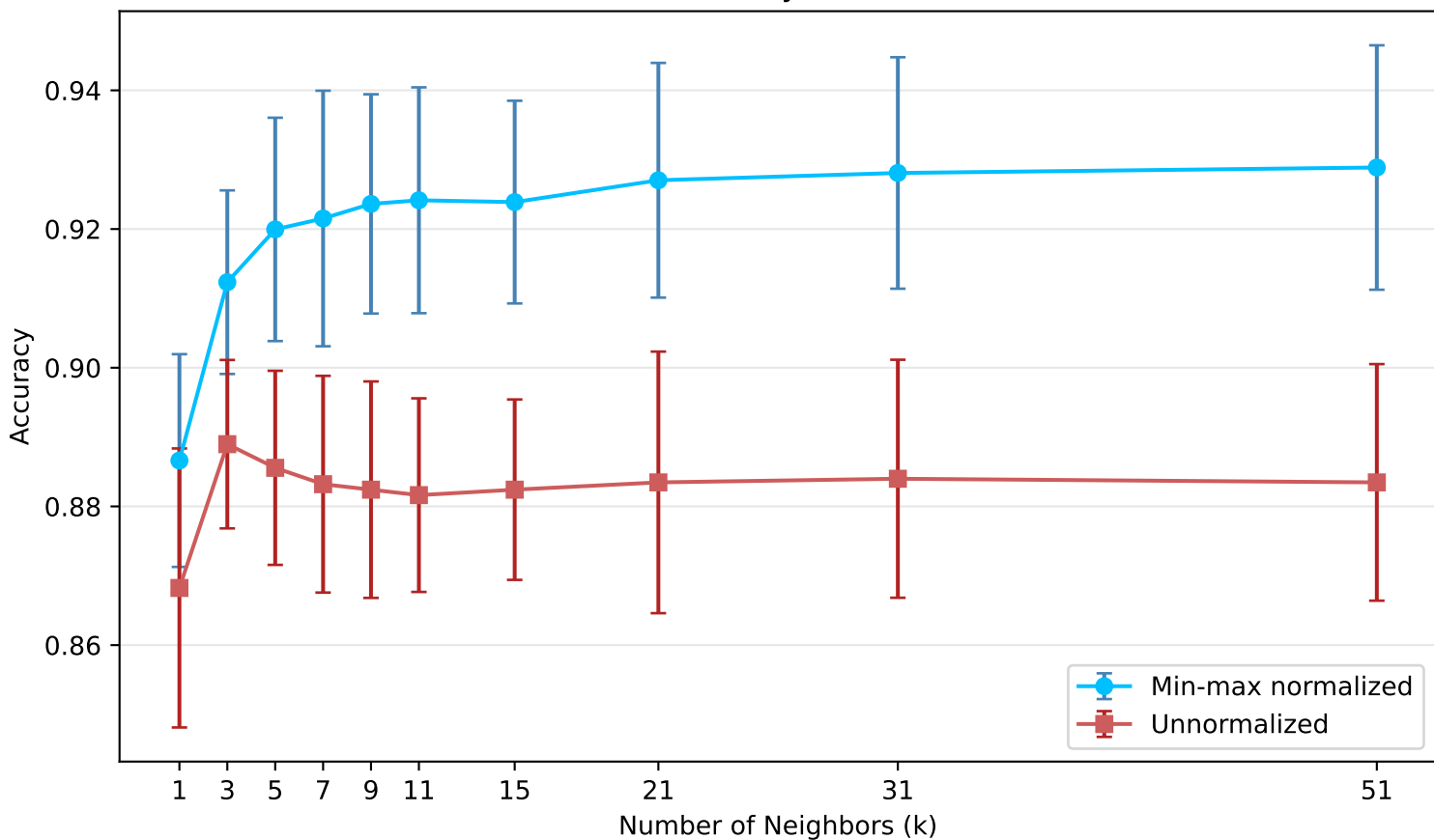
Dataset #1 (Rice): k-NN Accuracy with vs. without Normalization
