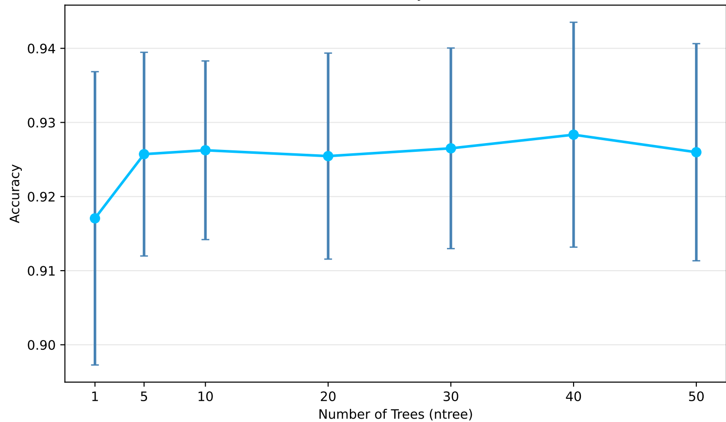
Dataset #1 (Rice): Accuracy vs. Number of Trees
