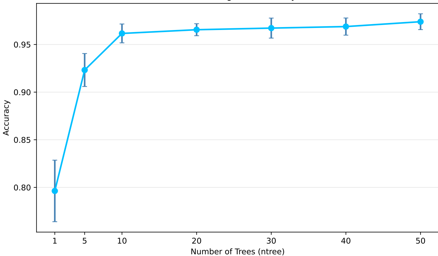
Dataset #1.1 (Hand-Written Digits): Accuracy vs. Number of Trees
