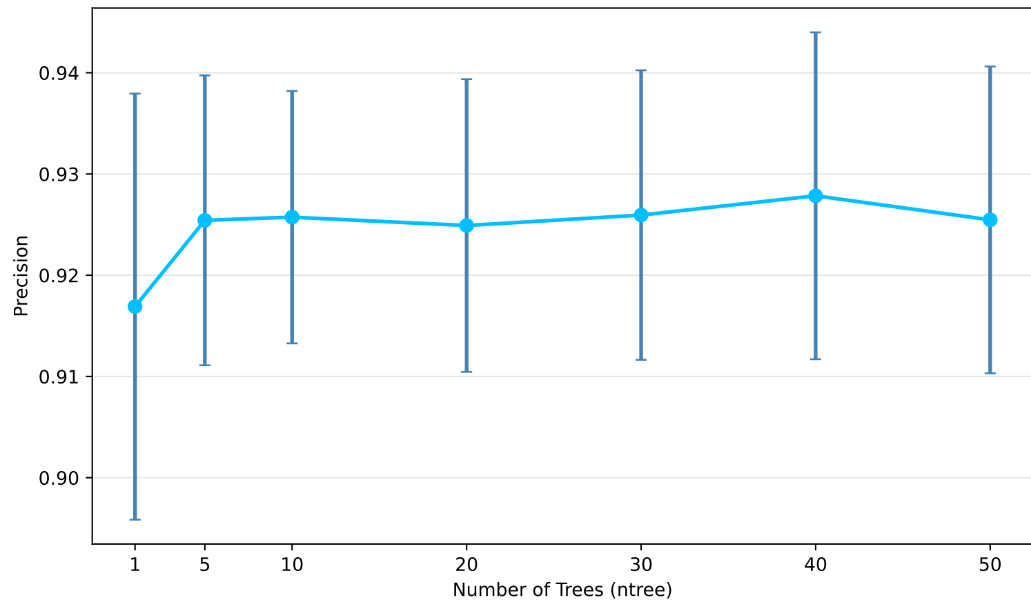
Dataset #1 (Rice): Precision vs. Number of Trees
