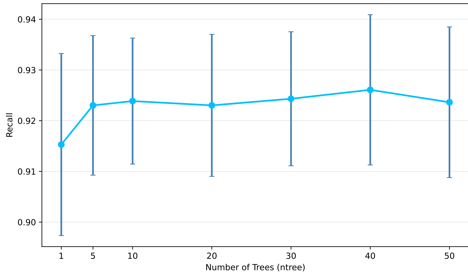
Dataset #1 (Rice): Recall vs. Number of Trees
