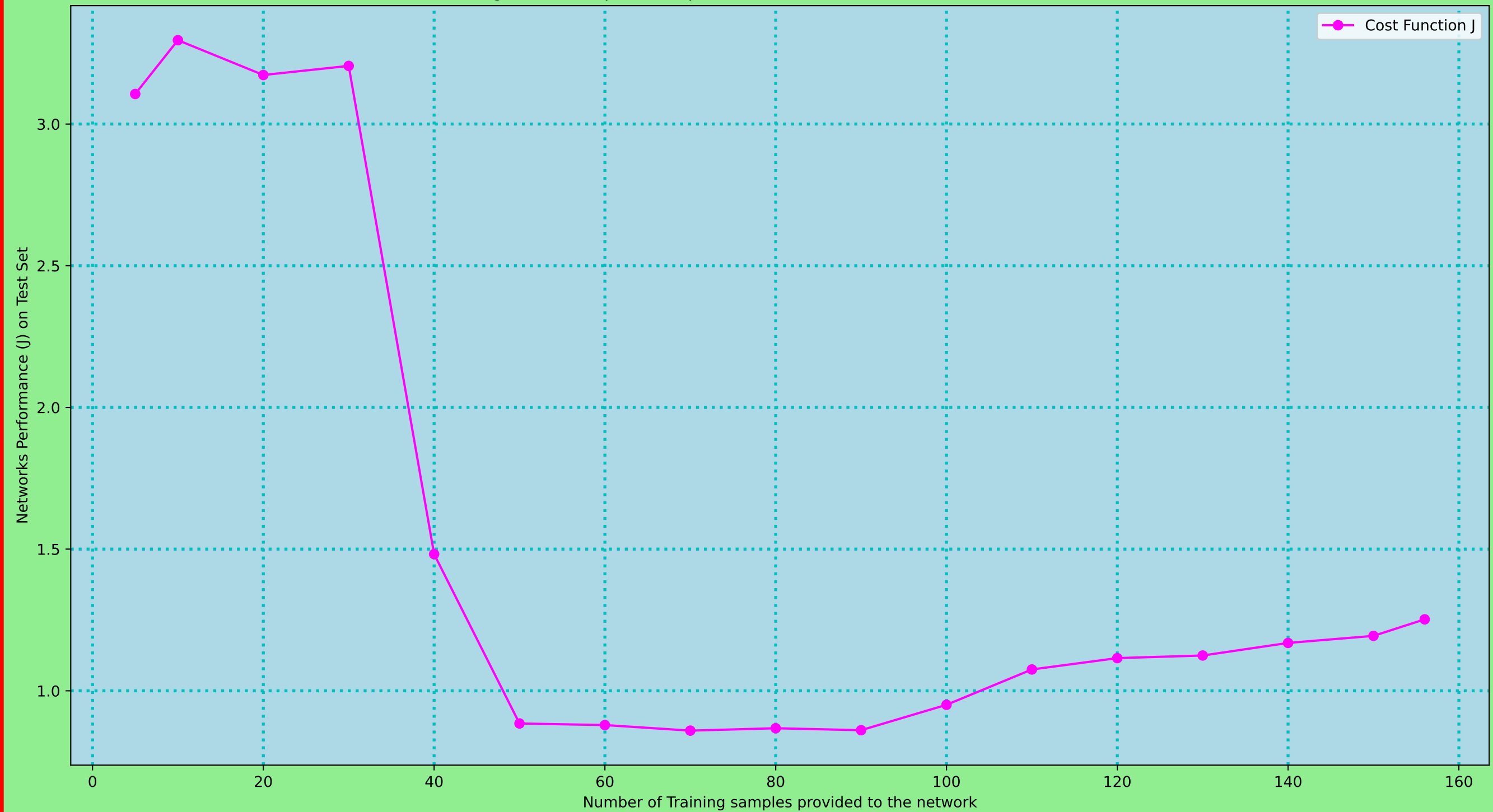
Parkinsons Disease Detection Dataset Learning Curve (Step Size (Alpha) = 0.05, Lambda \lambda = 0.01, m = 2000, Best Neural Network Architecture : [22, 3, 1])
