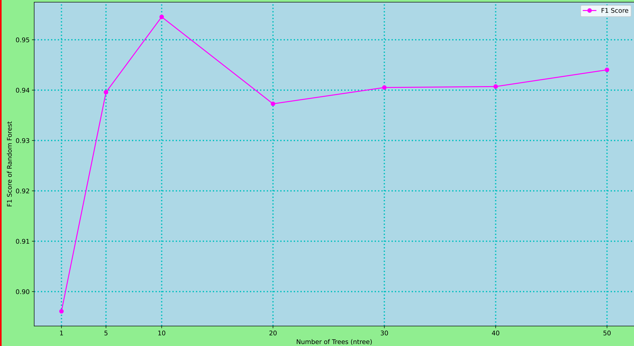
The Oxford Parkinson's Disease Detection Dataset - F1 Score of Random Forest as a function of ntree
