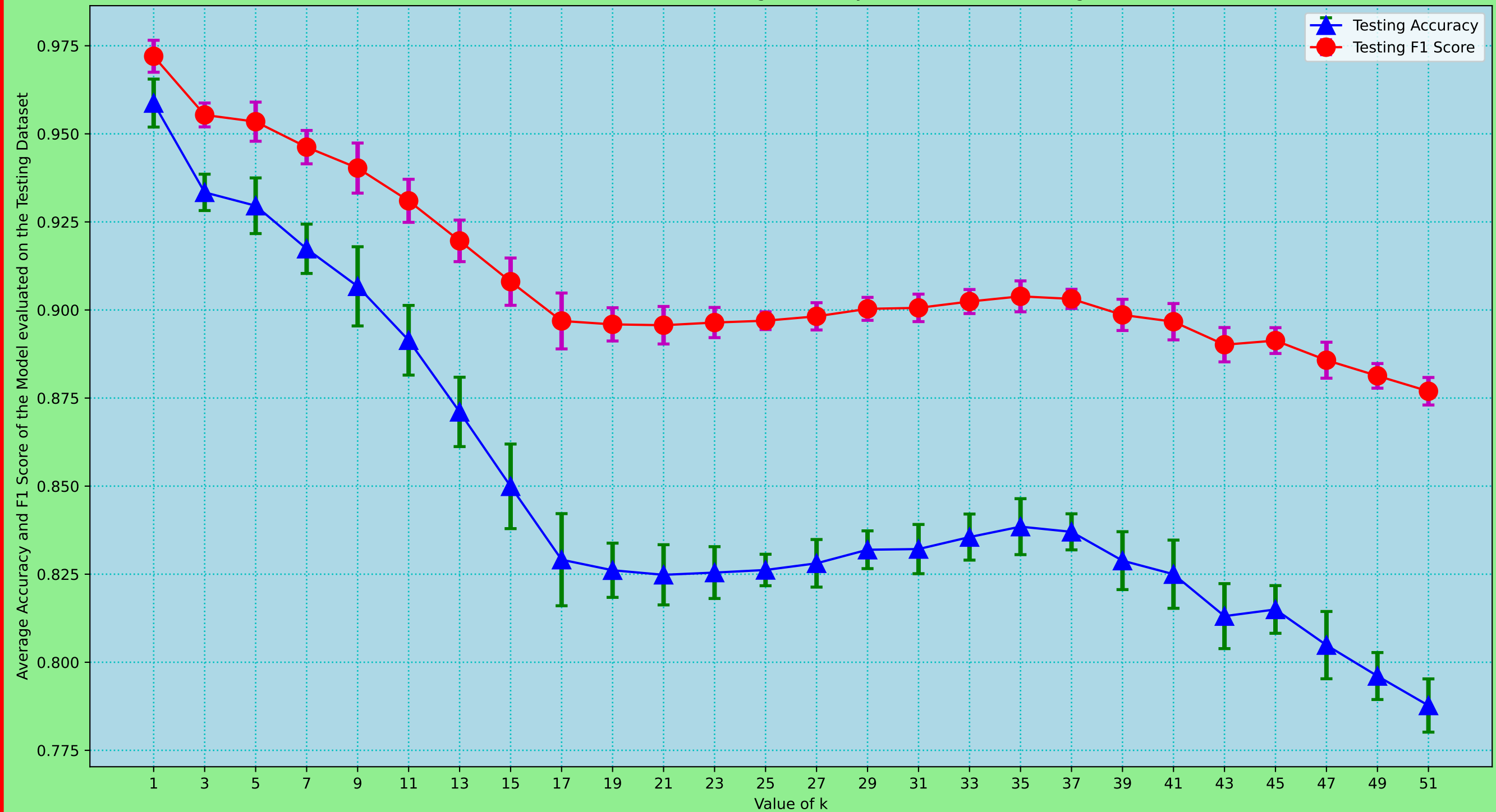
Parkinsons Disease Detection Dataset - K-NN Average Accuracy and F1 Score on Testing Dataset VS Value of k
