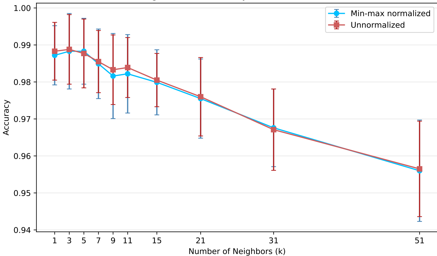
Dataset 1.1 (Digits): k-NN Accuracy with vs. without Normalization
