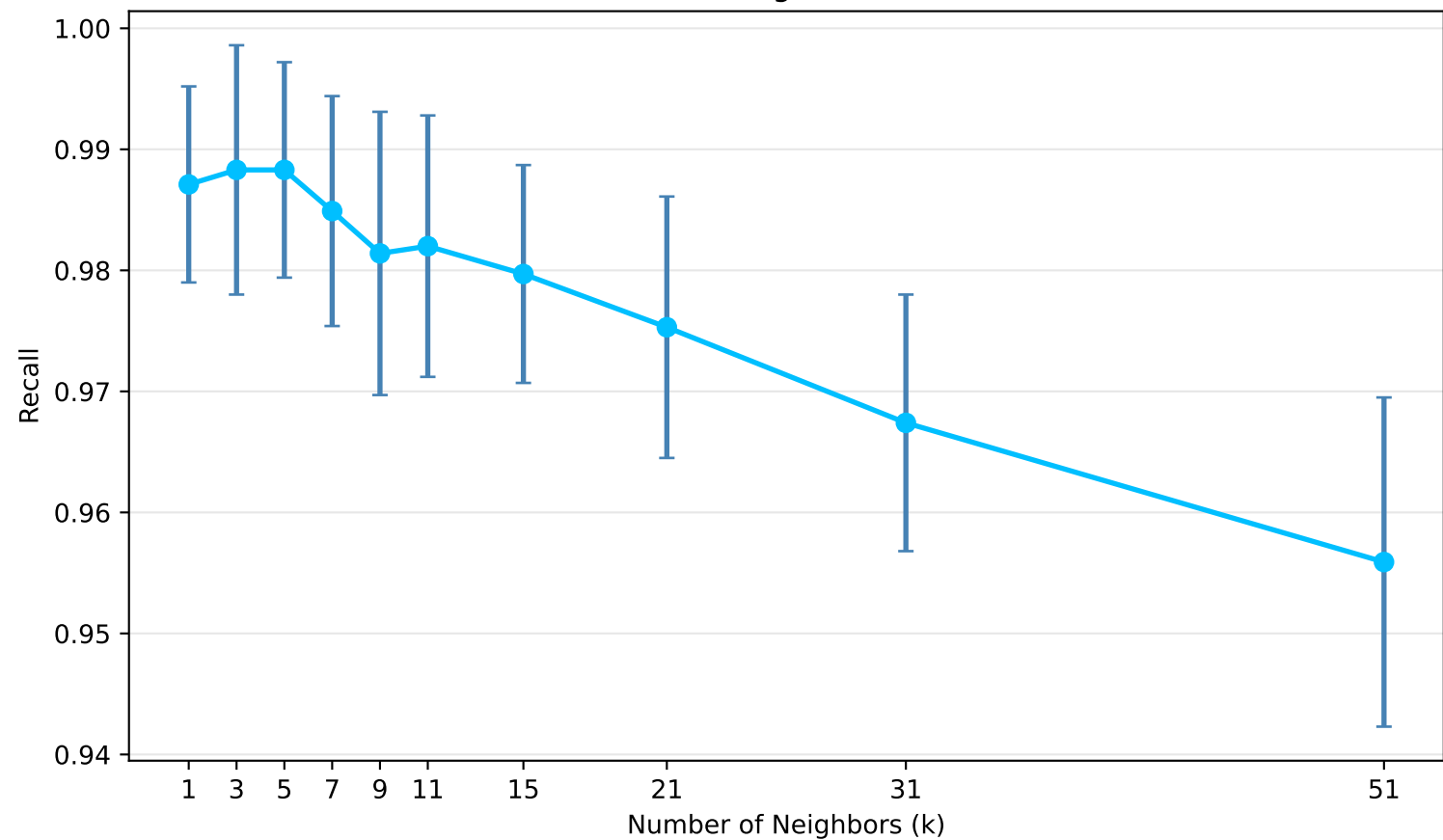
Dataset 1.1 (Digits): Recall vs. k
