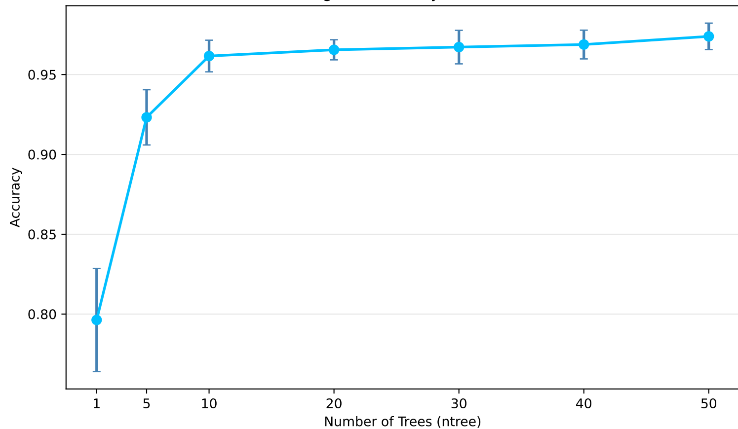
Dataset 1.1 (Digits): Accuracy vs. Number of Trees
