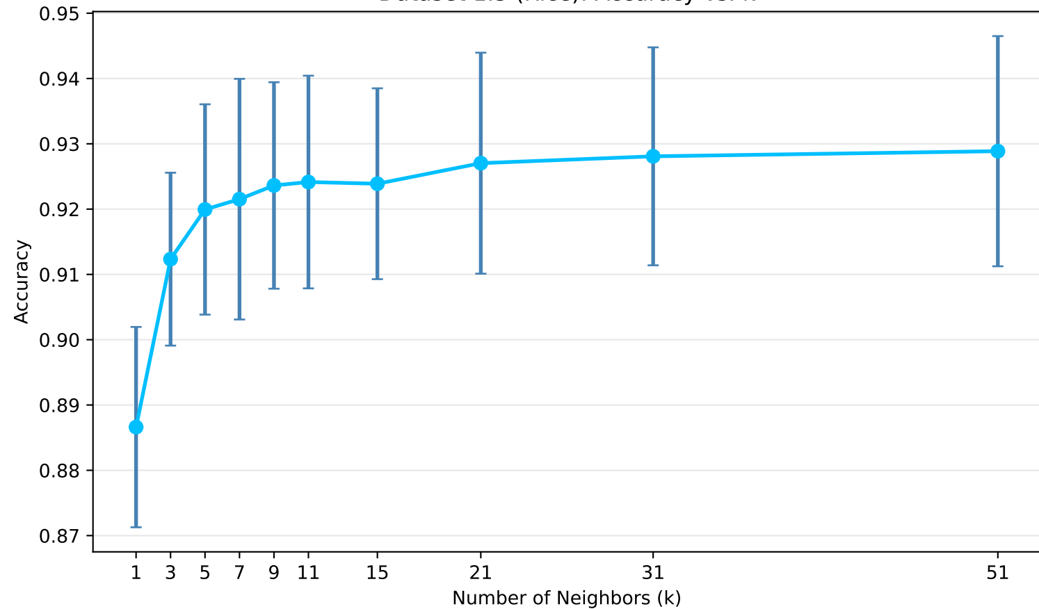
Dataset 1.3 (Rice): Accuracy vs. k
