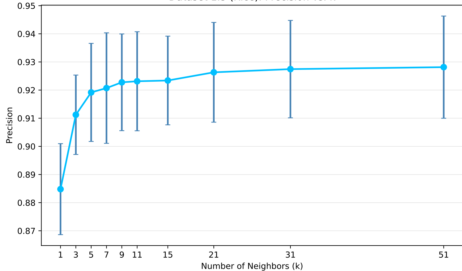
Dataset 1.3 (Rice): Precision vs. k
