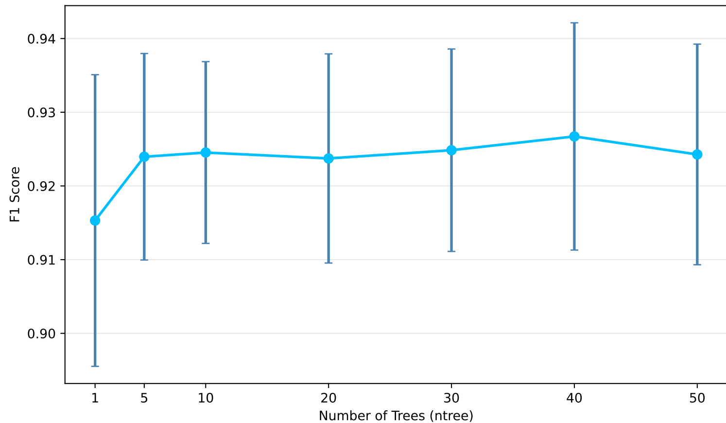
Dataset 1.3 (Rice): F1 Score vs. Number of Trees
