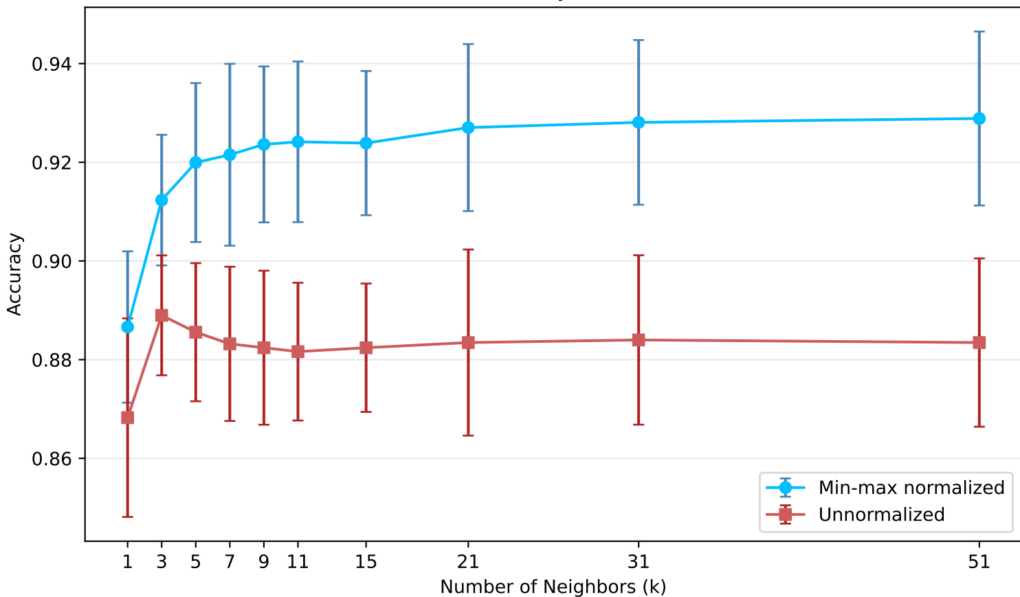
Dataset 1.3 (Rice): k-NN Accuracy with vs. without Normalization
