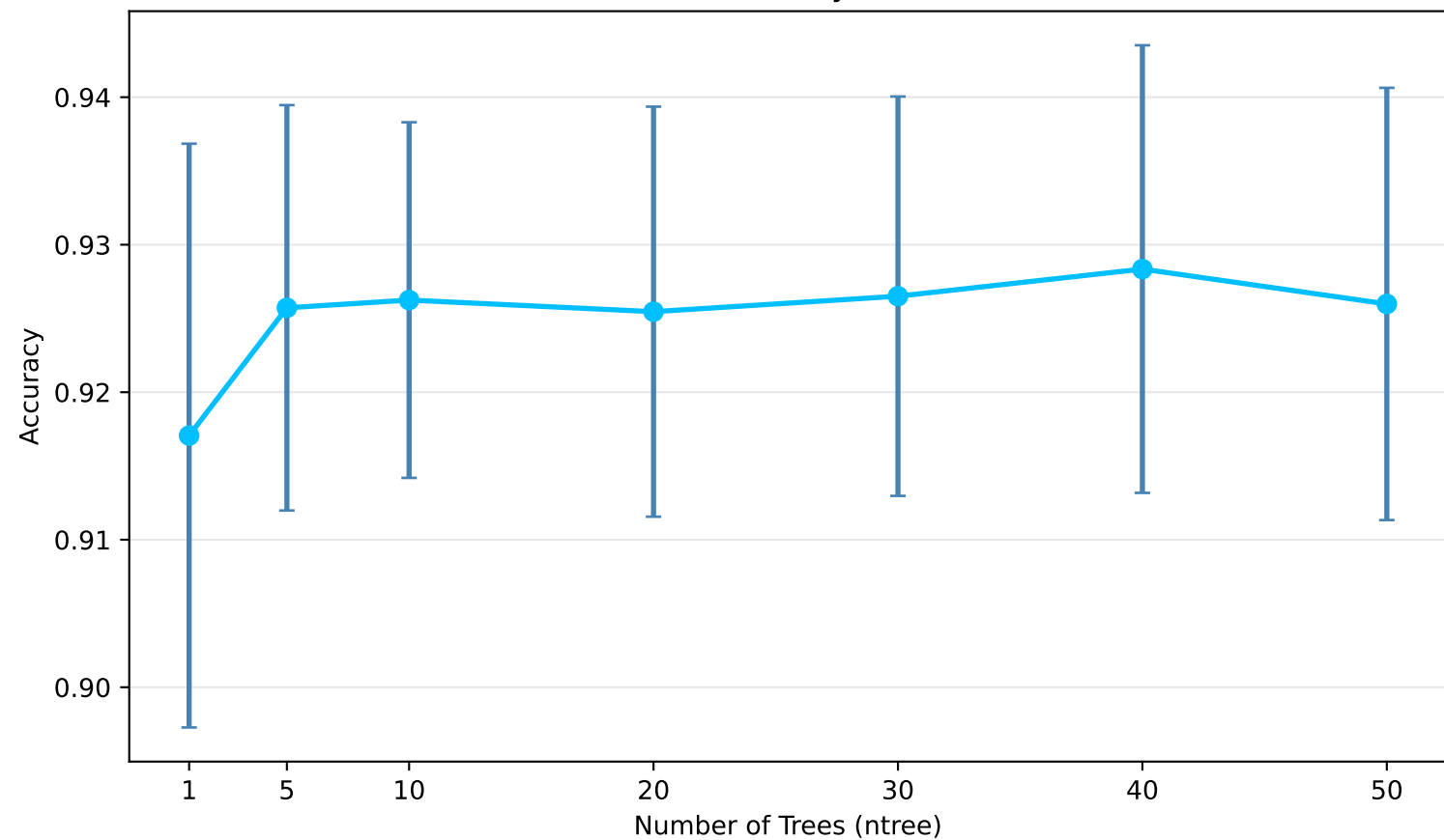
Dataset 1.3 (Rice): Accuracy vs. Number of Trees
