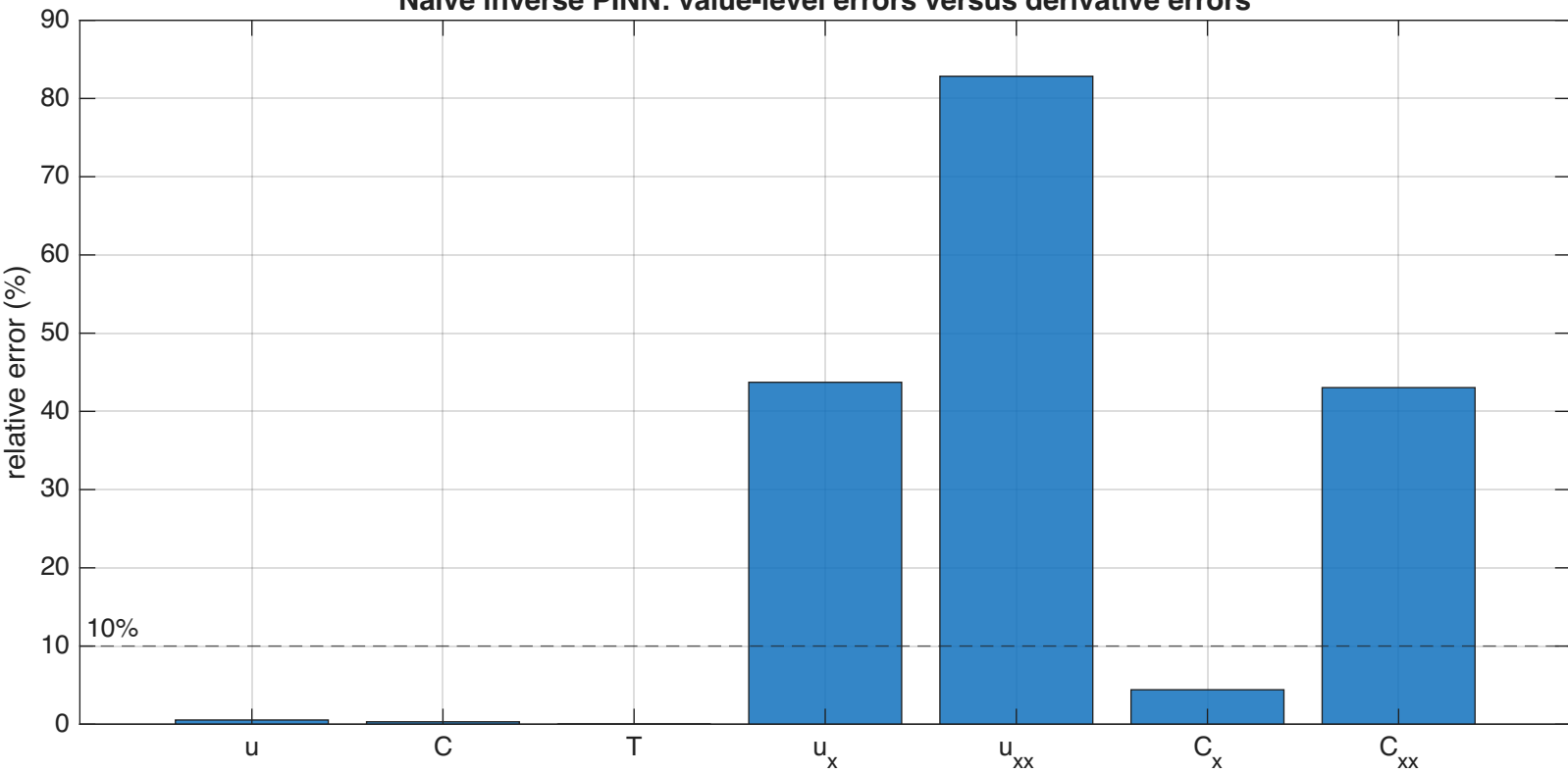
Naive inverse PINN: value-level errors versus derivative errors
