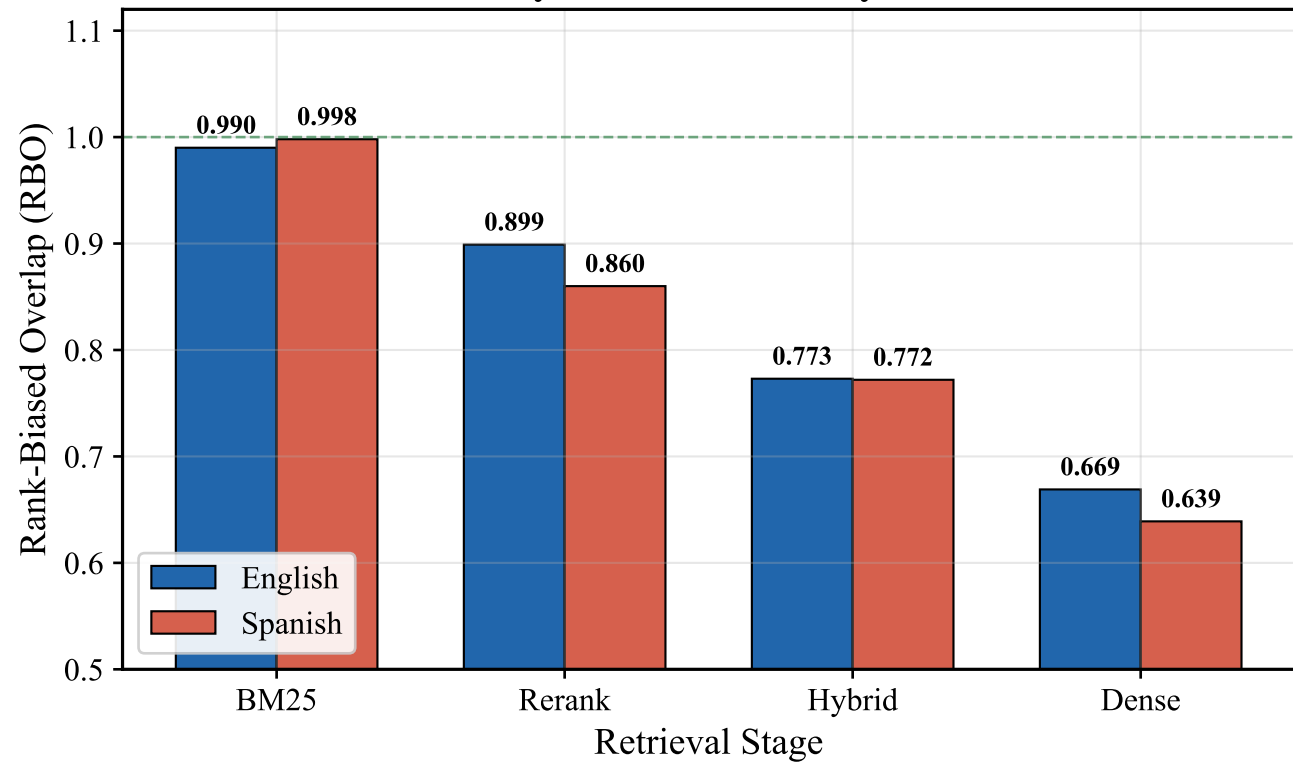
Rank Stability Under Name-Only Perturbation
