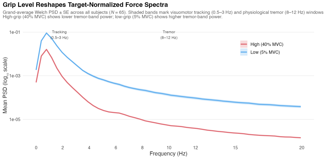
Figure 3: Grand-average Welch PSD \pm SE by grip condition. Shaded bands mark the tracking (0.5–3 Hz) and tremor (8–12 Hz) analysis windows.
