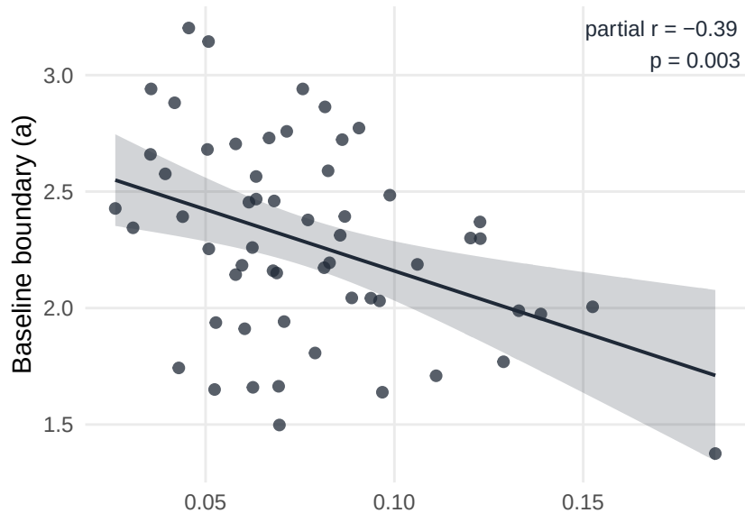
DDM baseline
