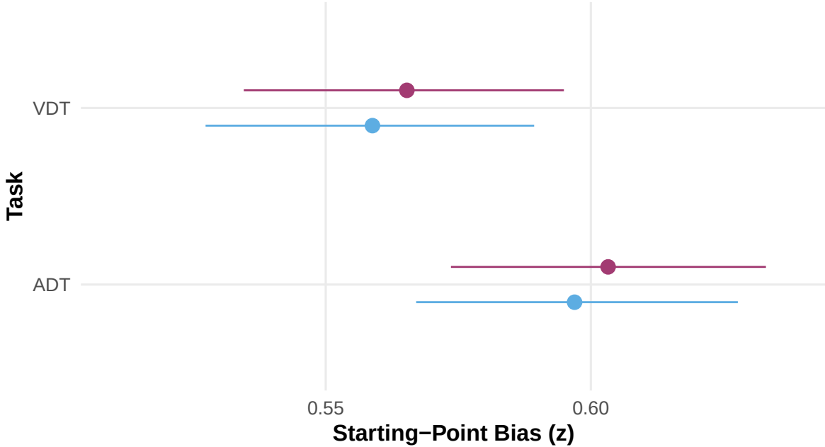
Standard-only model
