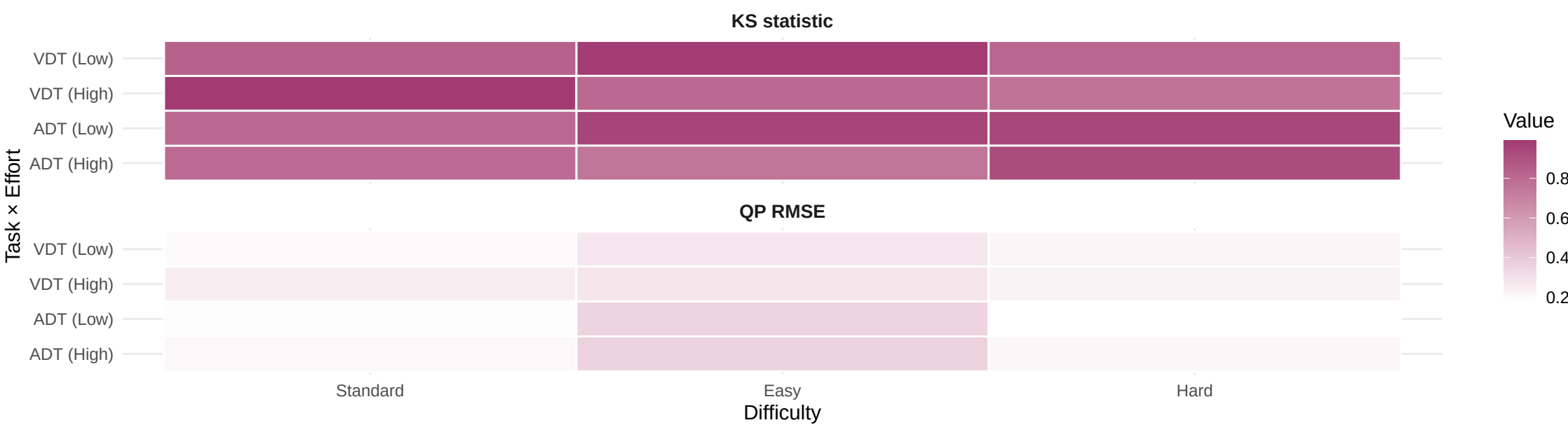
PPC Residual Heatmaps: Primary Model (Primary) KS statistic and QP RMSE by Task × Effort × Difficulty
