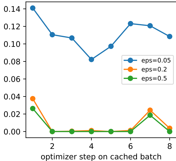
clip fraction (minibatch)
