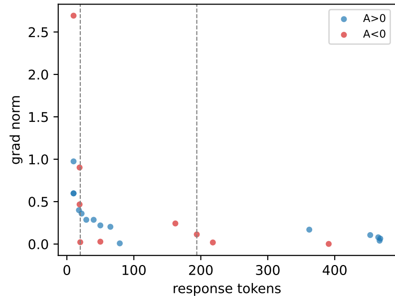
grpo: per-completion policy-gradient norm
