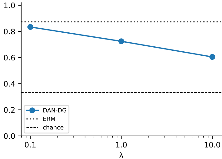
(b) 3-way source-domain separability
