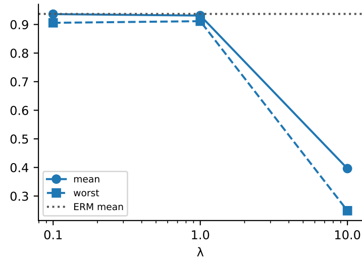
(a) source-val macro-F1
