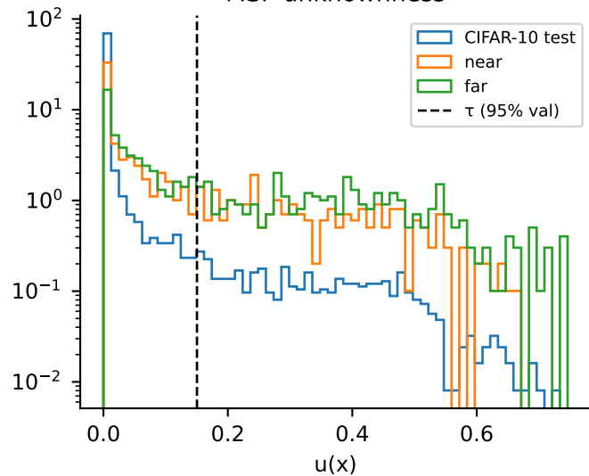
MSP unknownness
