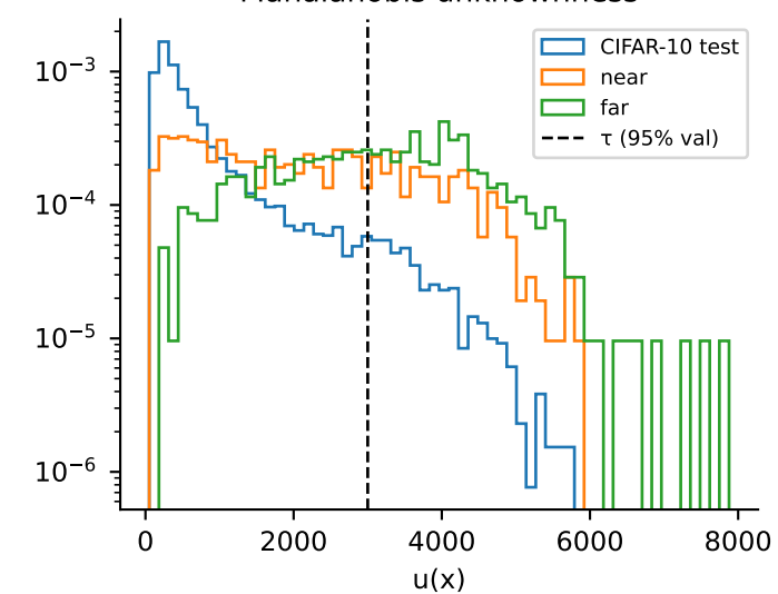
Mahalanobis unknownness
