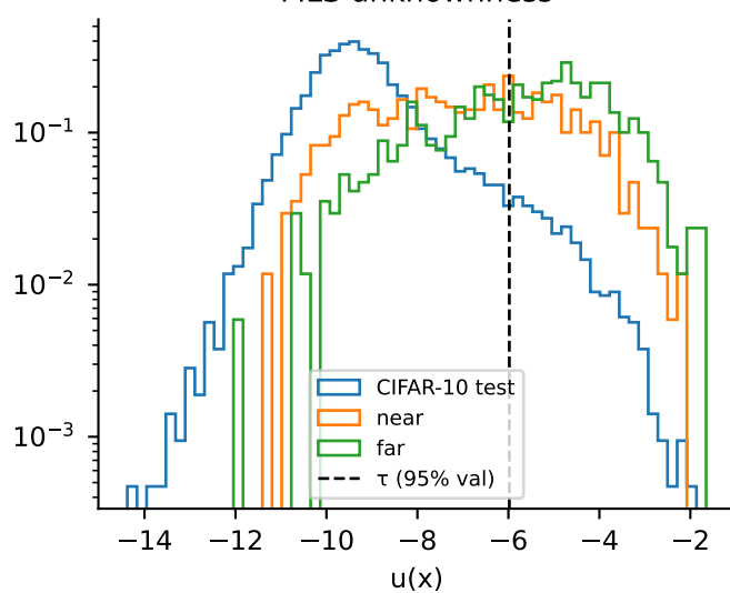
MLS unknownness
