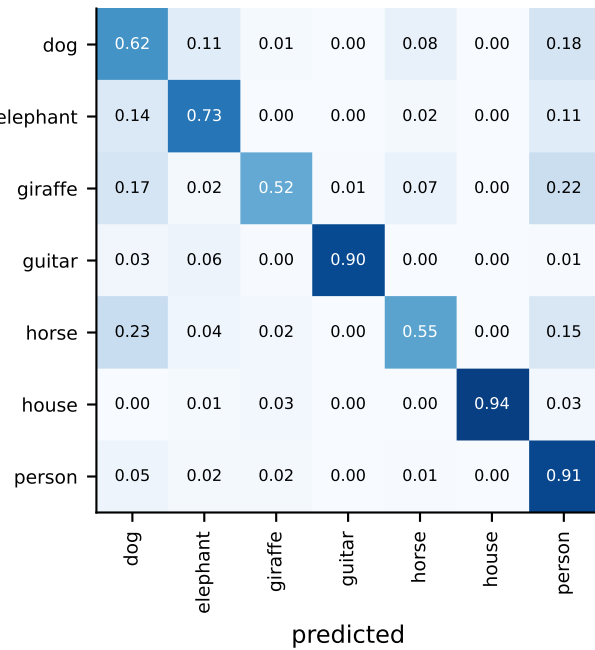
SAM ( \rho=0.05 ) (acc 0.668)
